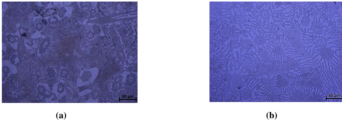
Fig. 1 Eutectic typical lamellar morphologies of Zn-Mg alloy solidified under (a) none electrical field and (b) positive electrical field ( E_+ = 14kVcm^{-1} ).
